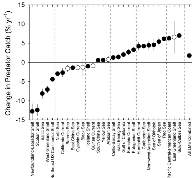
Fig. 2. Estimates of the instantaneous rate of change ( \% \text{ yr}^{-1} ) in apex predator catches ( \pm \text{SE} ) during the time period when the mean trophic level was declining in each ecosystem. Parameter estimates that are statistically different from zero ( P < 0.05 ) are indicated by filled circles, and estimates that are not significant are indicated by open circles. Under the sequential collapse/replacement mode ecosystems should show a large decline in apex predator catches, whereas under the sequential addition mode ecosystems should show no change or growth in apex predator catches.
