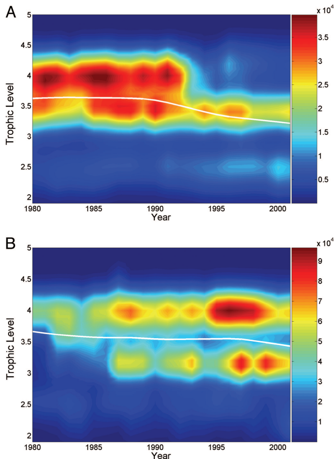
Fig. 1. Illustrative examples of the sequential collapse/replacement (A) and sequential addition (B) mode of fishing down the food web. Total yearly catch for each 0.1 trophic-level increment is indicated by the color bar on the right ( 10^4 \text{ kg yr}^{-1} ). The mean trophic level (white line) was smoothed by using a locally weighted regression smoother. (A) The Scotian Shelf ecosystem exhibited a sharp decline in mean trophic level from 1990 to 2001 owing to the collapse of the cod fishery followed by a decline in the herring fishery and then the growth of the northern prawn fishery. (B) The mean trophic level of the Patagonian Shelf declined from 1980 to 2001, during which time catches for upper-trophic-level species (Argentine hake) grew substantially while new fisheries for shortfin squid developed.
